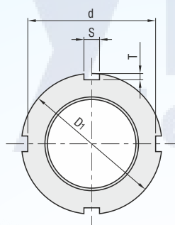
Bearing Nut
