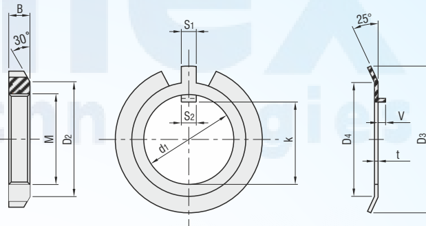
Tooth Lock Washer for Bearing
