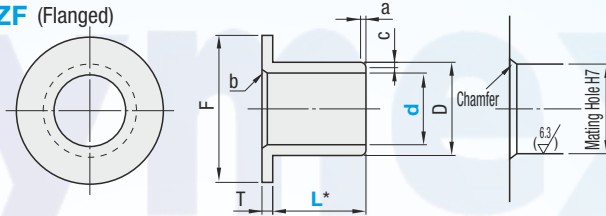
DJZF (Flanged)
