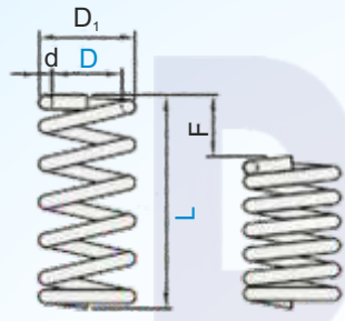
Closed End (* Dimensions Both Ends Not Ground)
