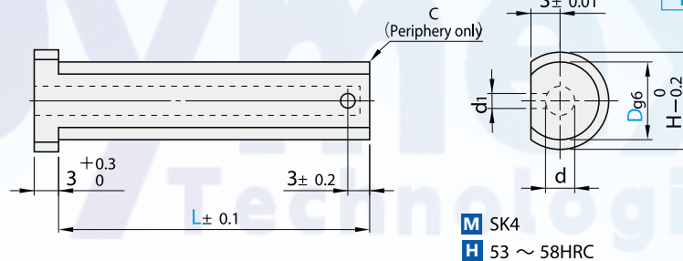
DLJS (Lifter pin with air hole)
