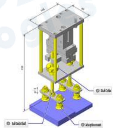
Example Use of Shaft Collars
