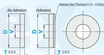
D,V Tolerance
